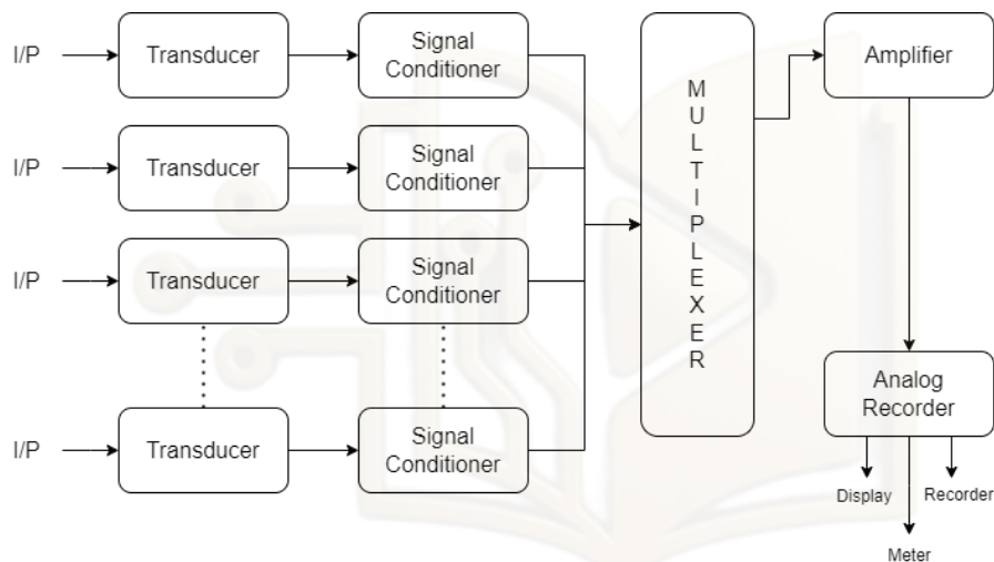
Fig: Analog Data Acquisition System
