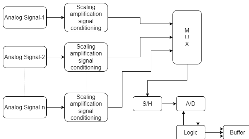
Fig: Multi-Channel Data Acquisition System
