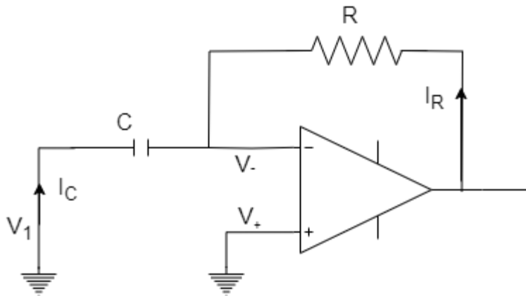
Fig: Operational Amplifier as Differentiation
