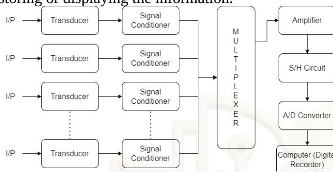
Fig: Digital Data Acquisition System
