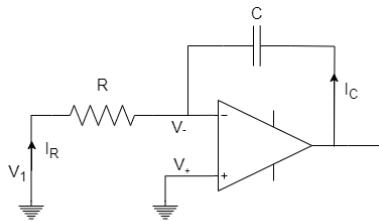
Fig: Operational Amplifier as Integrator
