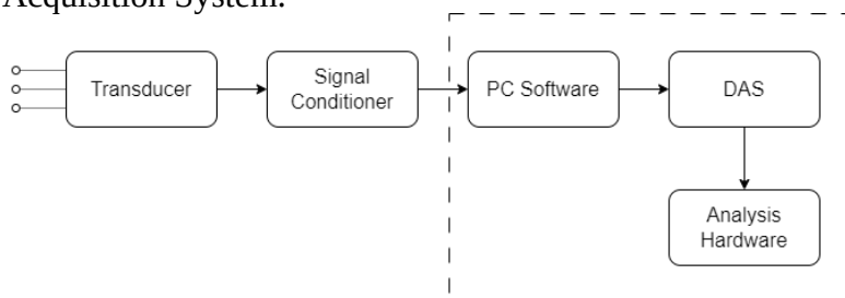
Fig: PC-BAsed Data Acquisition System
