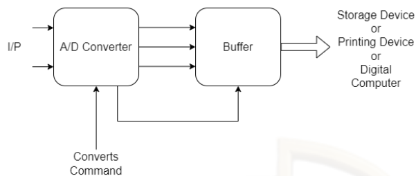
Fig: Single Channel Data Acquisition System
