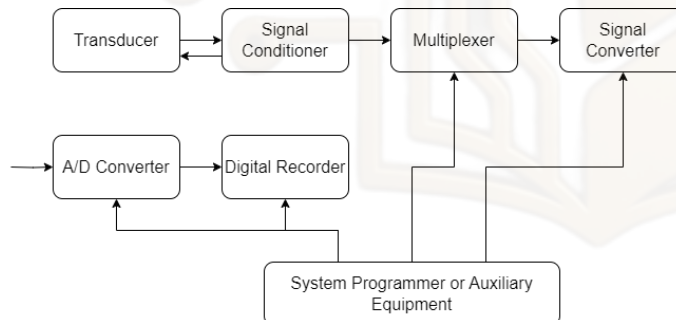
Fig: Modern Digital Data Acquisition System
